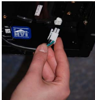
upgraded capacitor and wiring inside easy-to-remove harness and quick-release Molex connector from power supply
